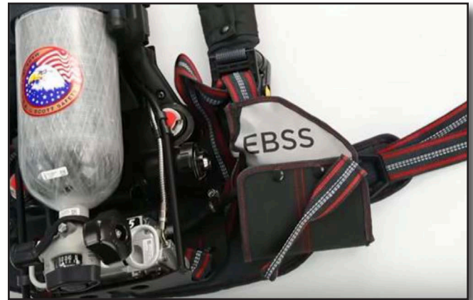
Figure 6-17 EBSS Pouch Location on SCBA
