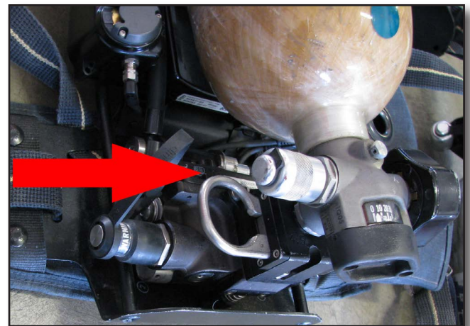
Figure 6-7 Pressure Reducer
