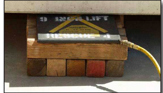
Figure 25-29 Solid Crib Bed for Achieving Maximum Airbag Lift
