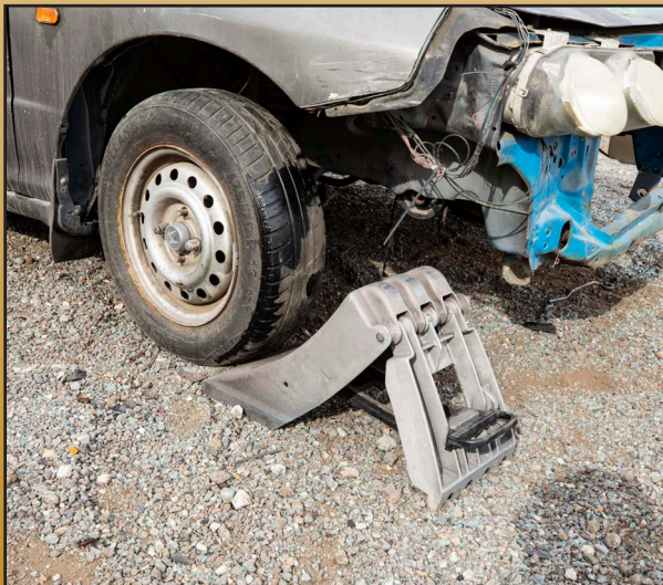
3. Stabilize wheels with cribbing or wheel chocks
