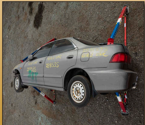
4. Vehicle is stabilized utilizing a 4 strut tension buttress system
