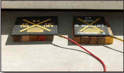
Figure 25-28 Side-By-Side Two Bag Lift
