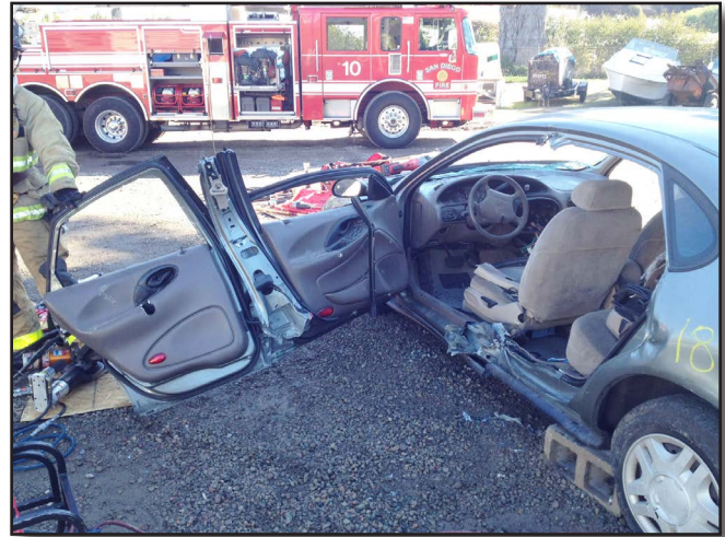
Figure 25-21 “B” Post Blow-Out (method 2)
