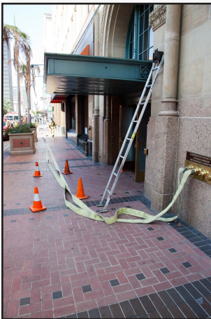
Figure 31-53 Connect a minimum of two supply lines to the FDC and set up two engine companies to pump in series.
